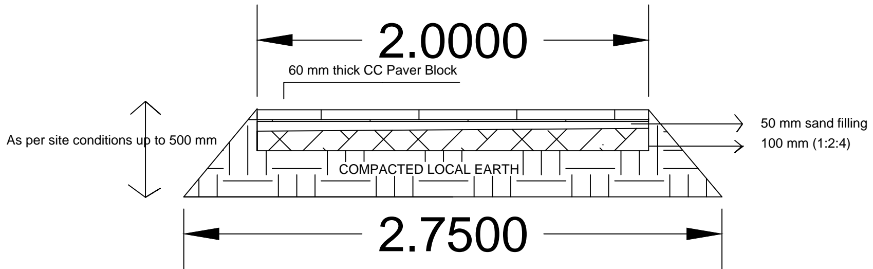
Typical Section of C.C Paver Block Pathway for 12 mtrs R.O.W
