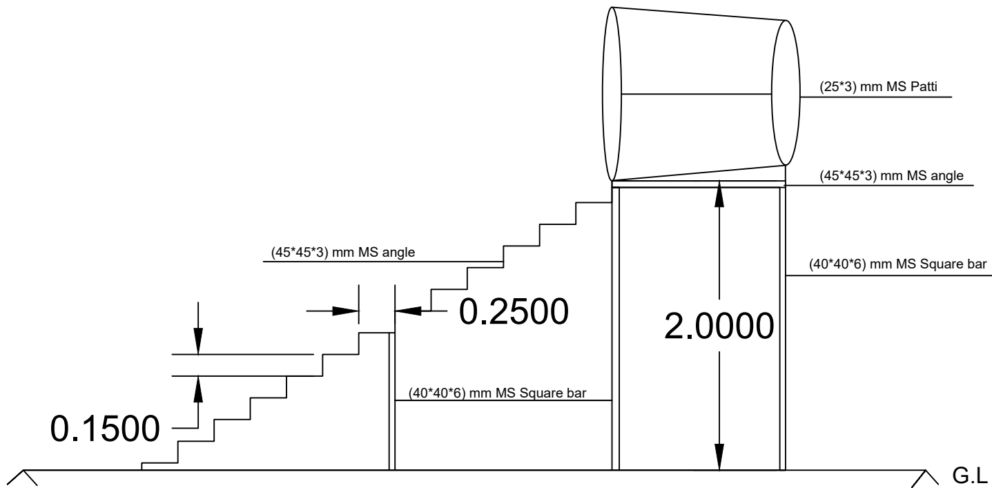
SIDE VIEW OF FLOWER RACK
